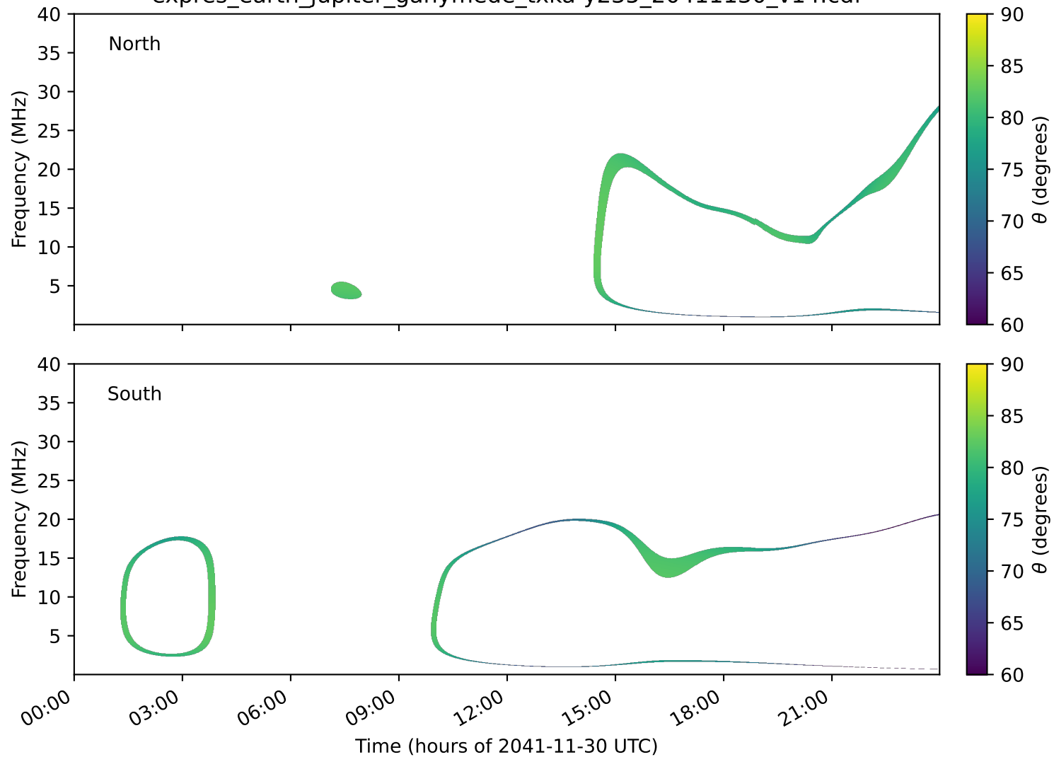
expres_earth_jupiter_ganymede_txka-y235_20411130_v14.cdf
