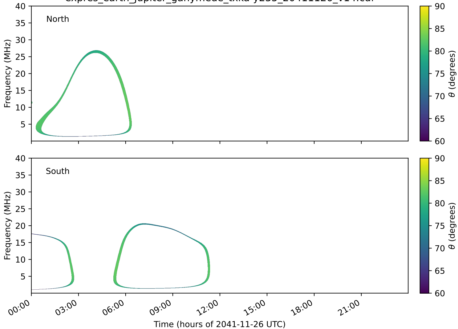
expres_earth_jupiter_ganymede_txka-y235_20411126_v14.cdf
