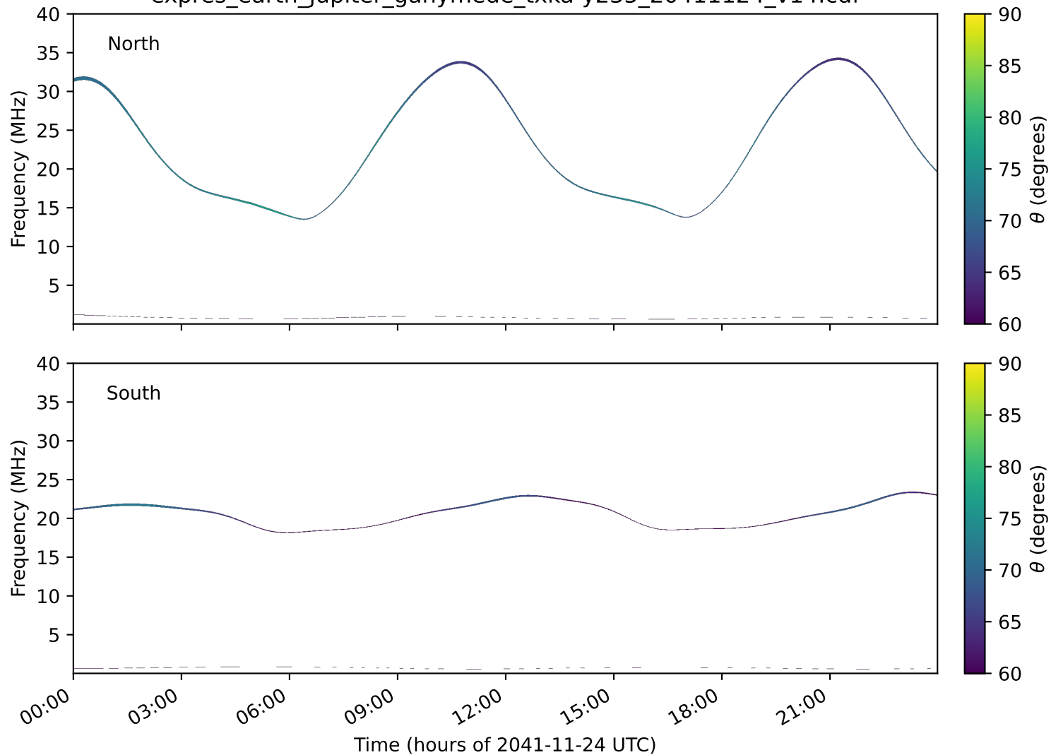
expres_earth_jupiter_ganymede_txka-y235_20411124_v14.cdf
