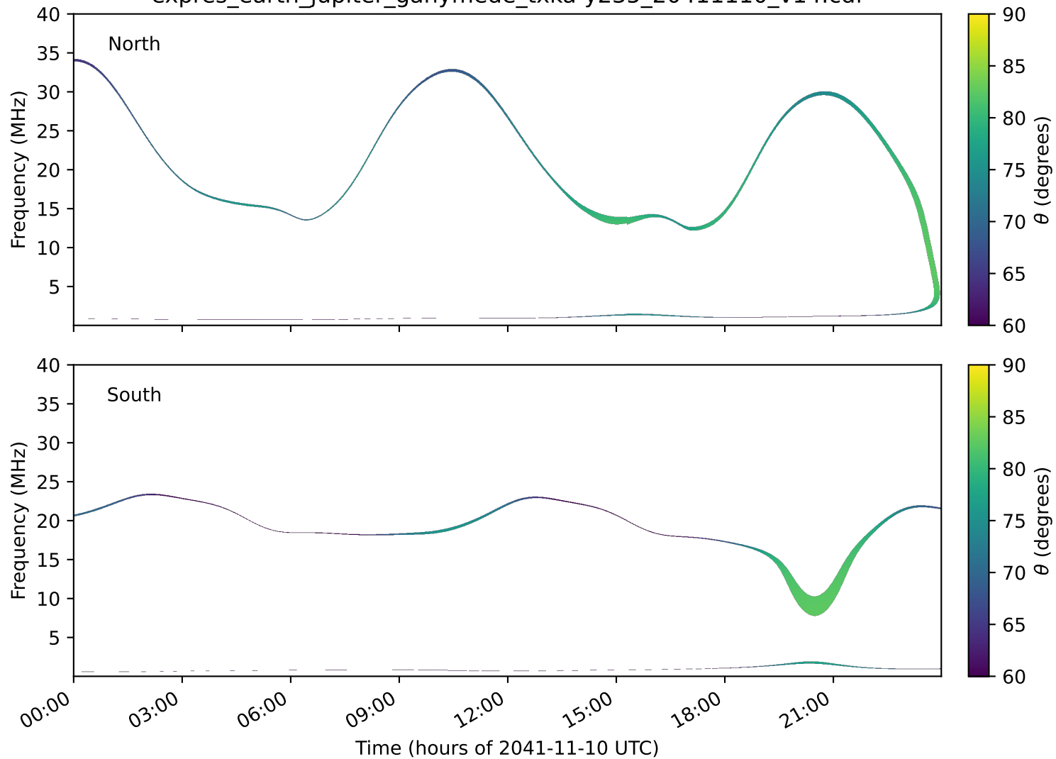
expres_earth_jupiter_ganymede_txka-y235_20411110_v14.cdf
