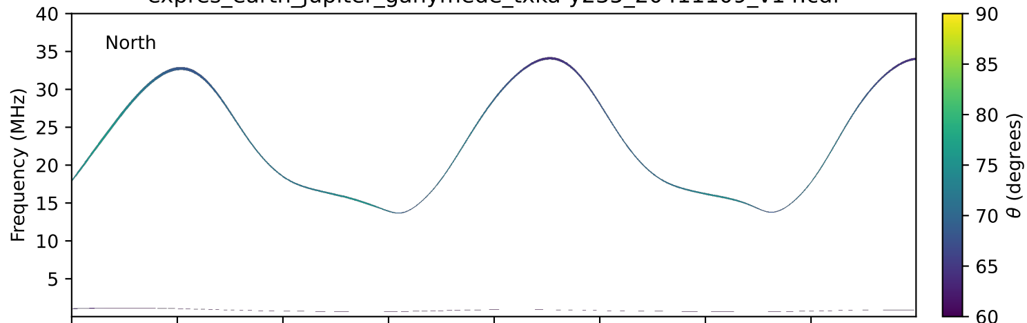
expres_earth_jupiter_ganymede_txka-y235_20411109_v14.cdf
