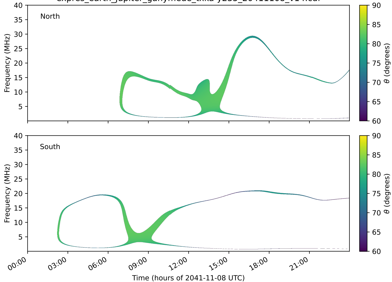
expres_earth_jupiter_ganymede_txka-y235_20411108_v14.cdf
