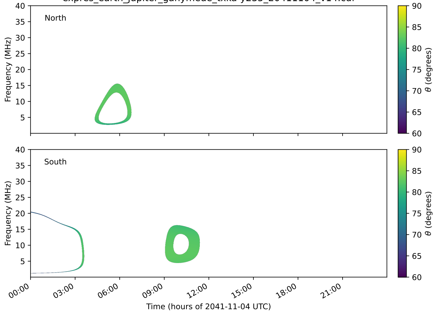
expres_earth_jupiter_ganymede_txka-y235_20411104_v14.cdf
