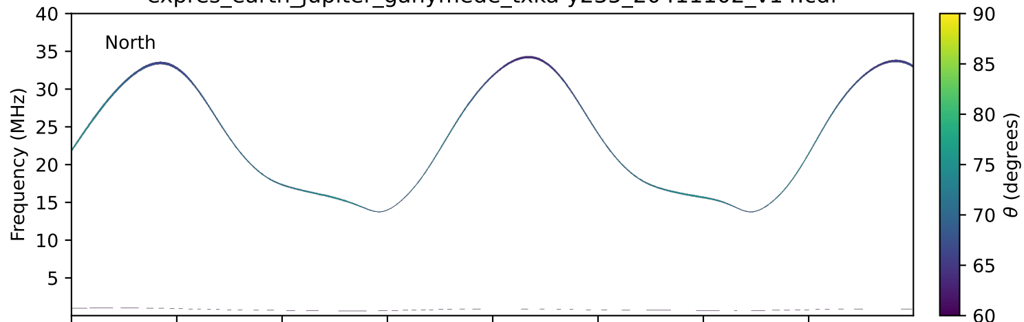
expres_earth_jupiter_ganymede_txka-y235_20411102_v14.cdf
