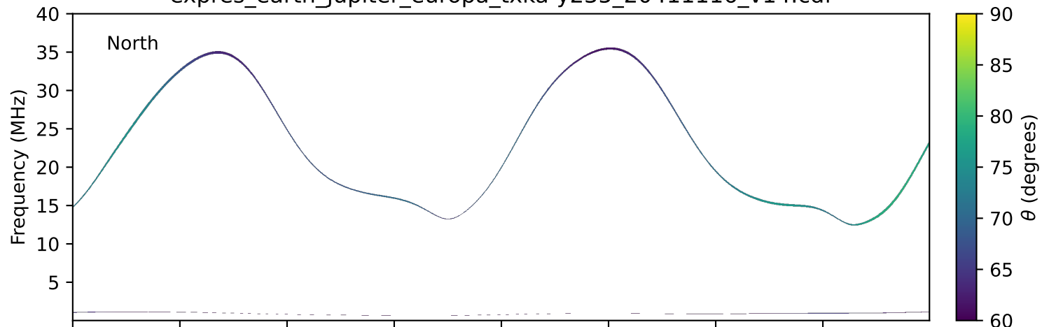
expres_earth_jupiter_europa_txka-y235_20411116_v14.cdf
