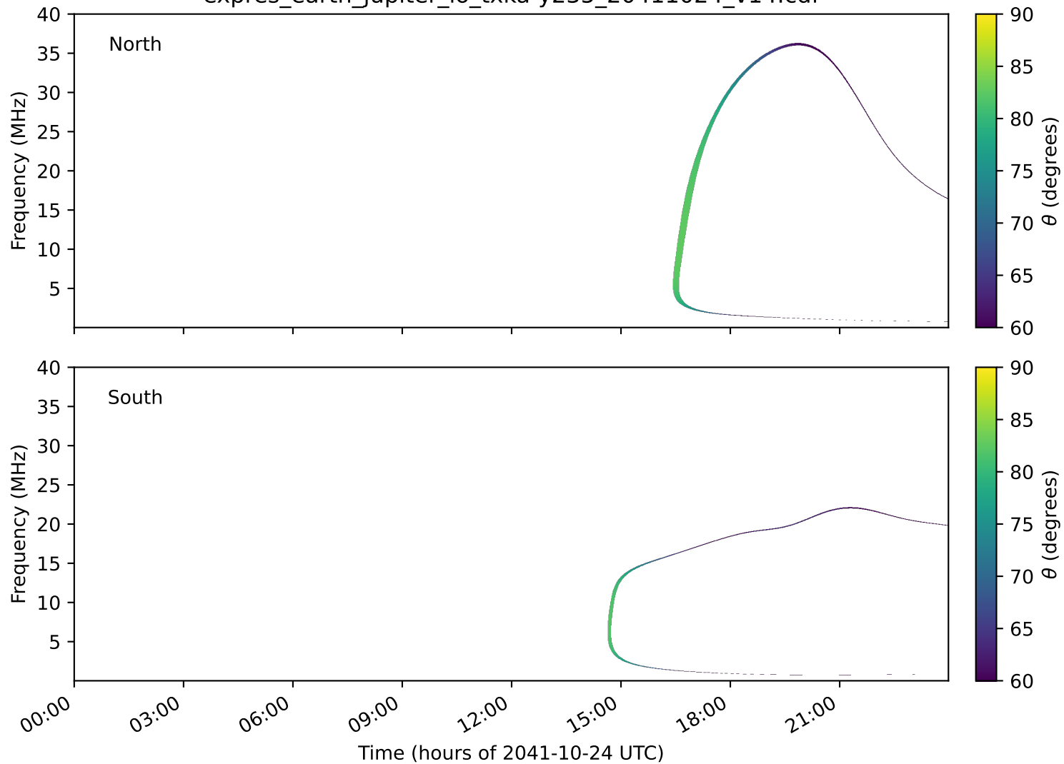
expres_earth_jupiter_io_txka-y235_20411024_v14.cdf
