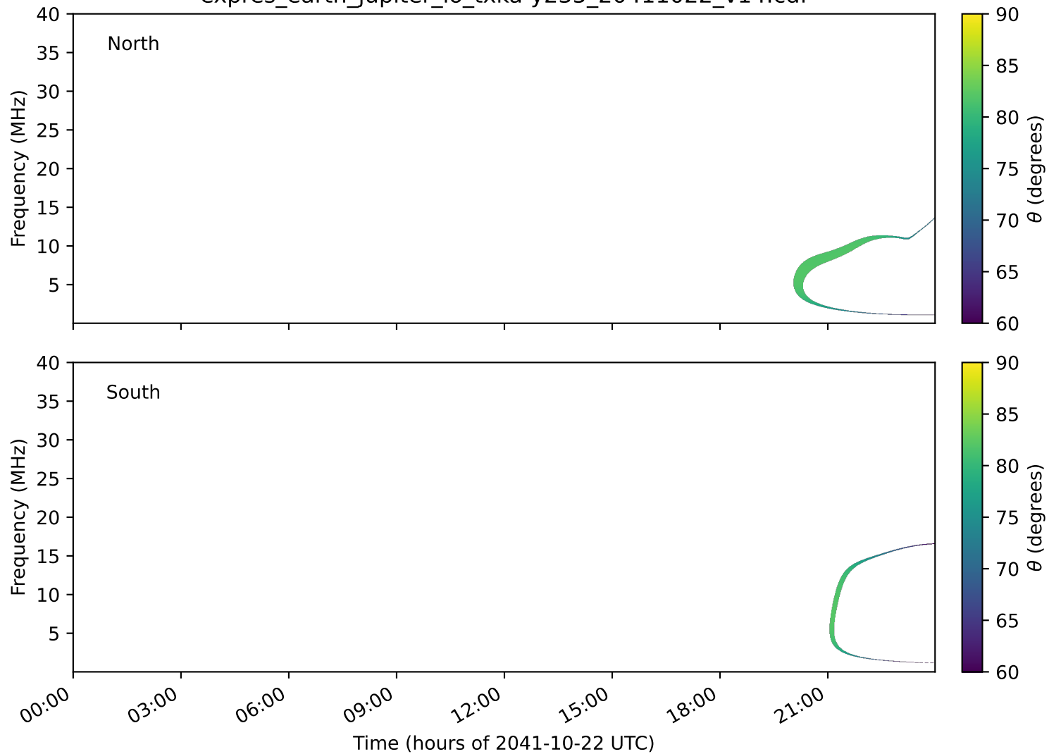
expres_earth_jupiter_io_txka-y235_20411022_v14.cdf
