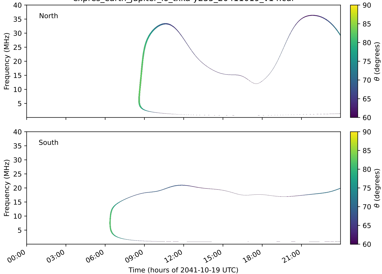
expres_earth_jupiter_io_txka-y235_20411019_v14.cdf
