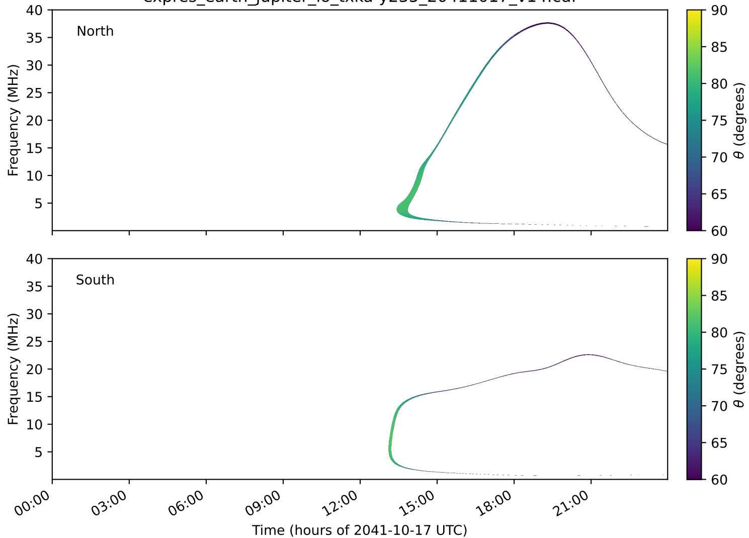
expres_earth_jupiter_io_txka-y235_20411017_v14.cdf
