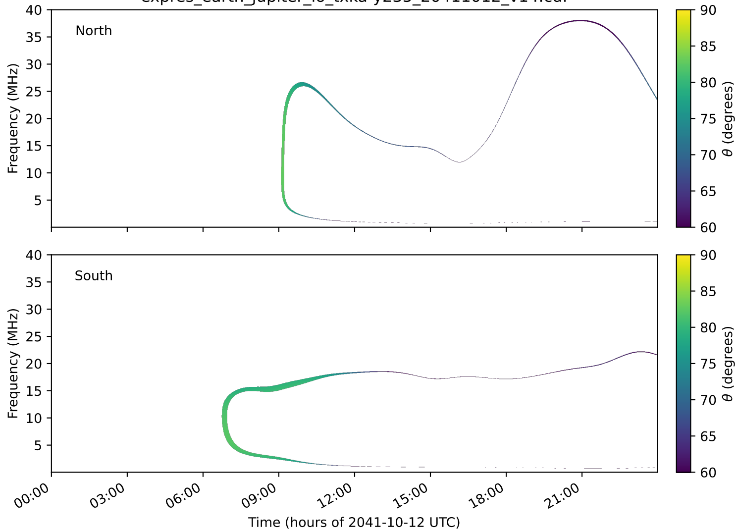
expres_earth_jupiter_io_txka-y235_20411012_v14.cdf
