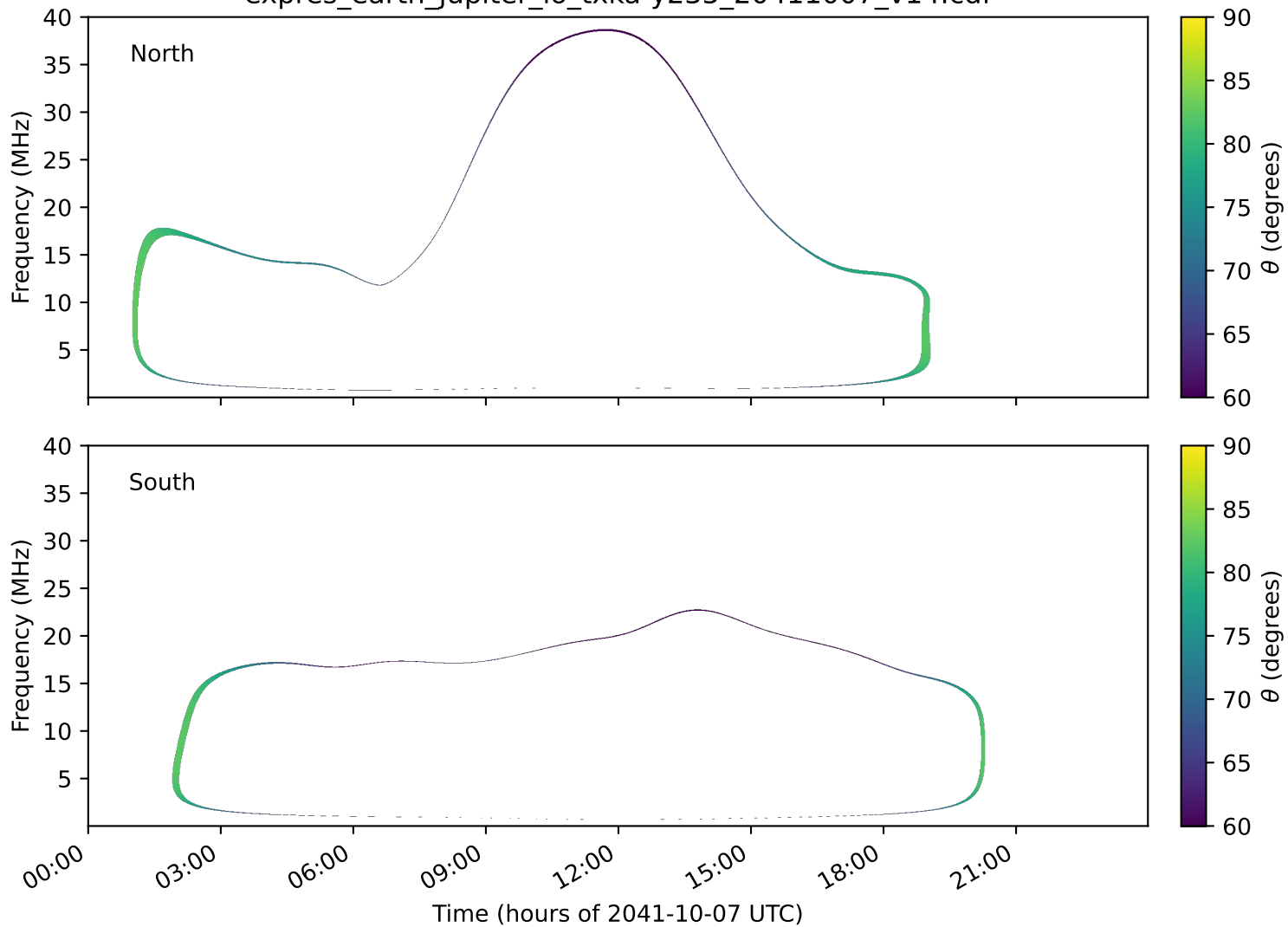
expres_earth_jupiter_io_txka-y235_20411007_v14.cdf
