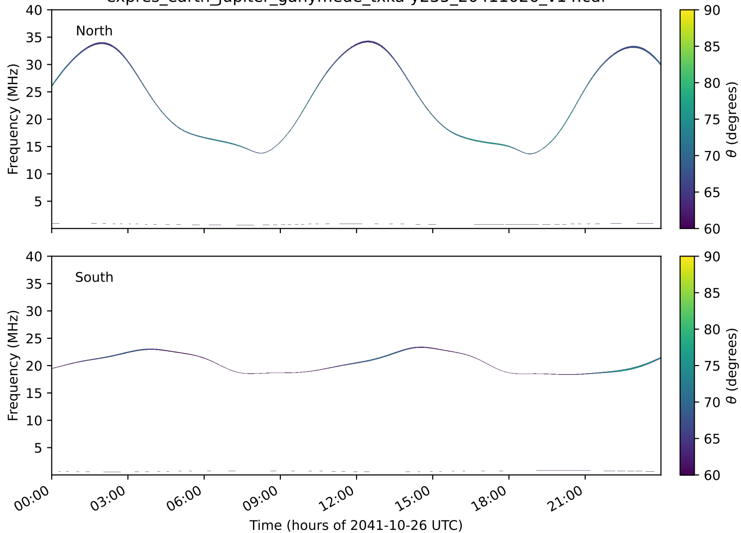
expres_earth_jupiter_ganymede_txka-y235_20411026_v14.cdf
