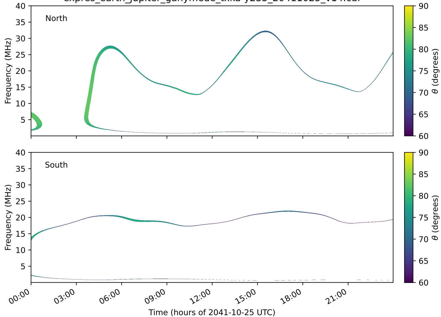
expres_earth_jupiter_ganymede_txka-y235_20411025_v14.cdf
