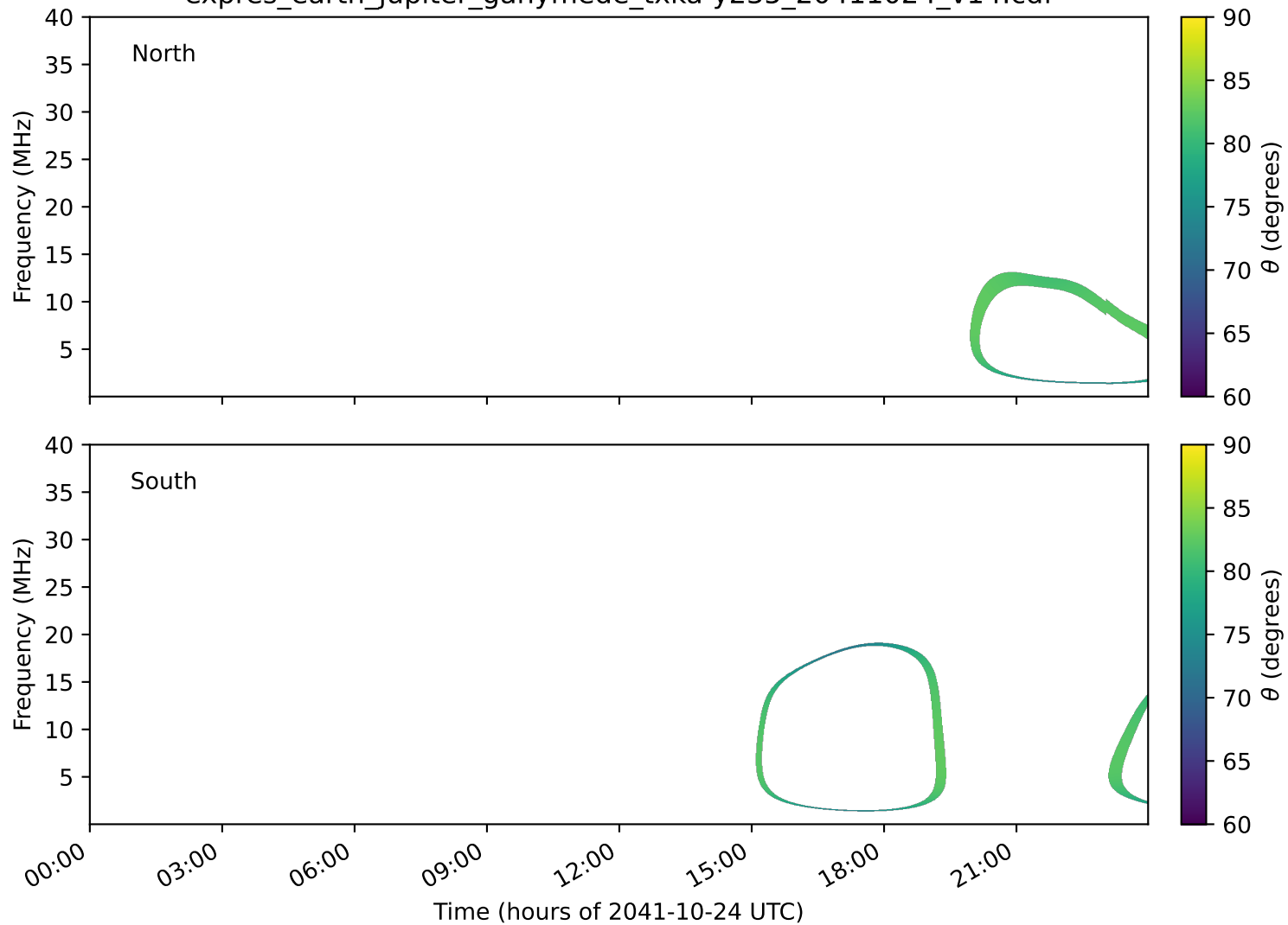
expres_earth_jupiter_ganymede_txka-y235_20411024_v14.cdf
