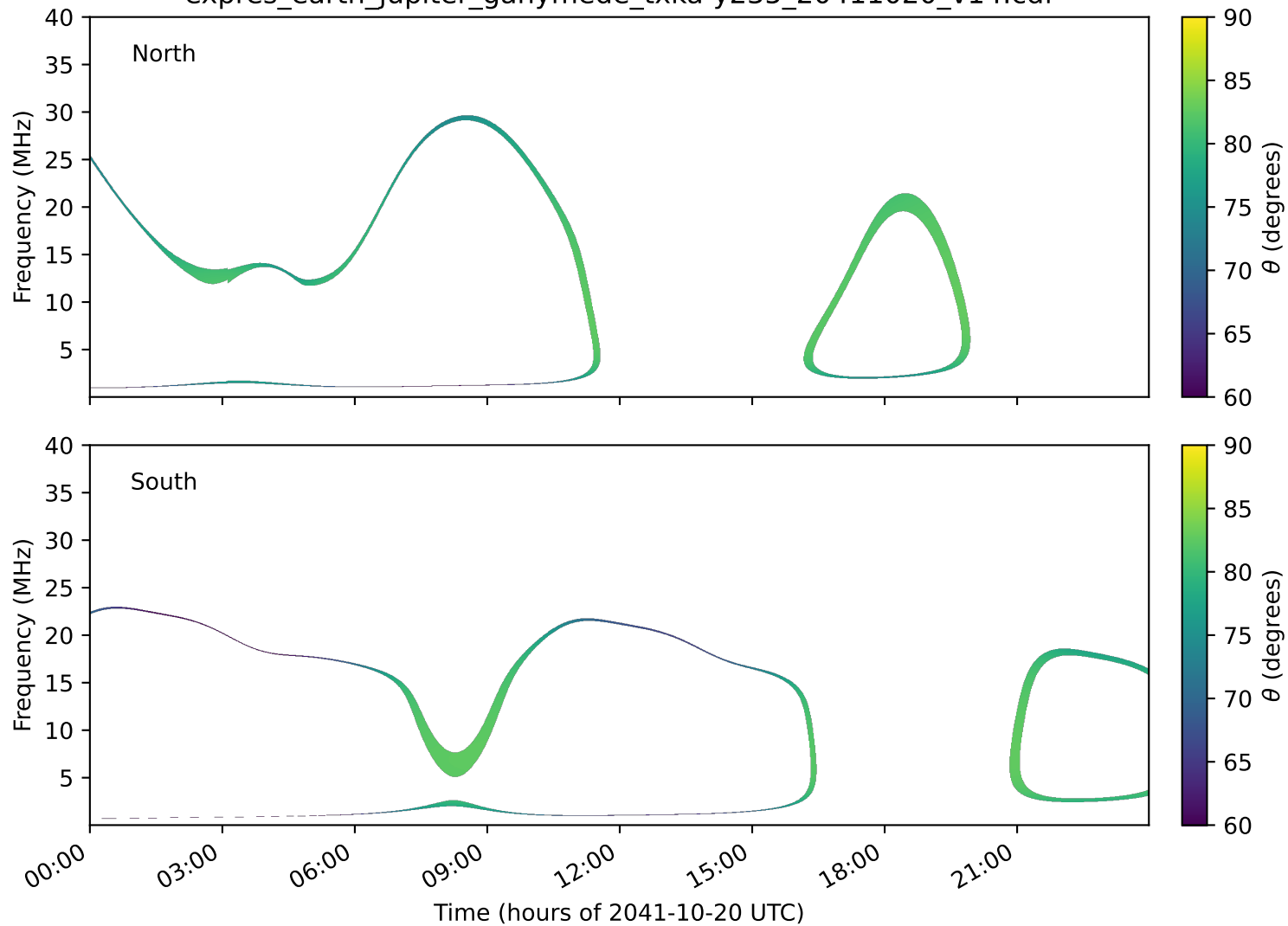
expres_earth_jupiter_ganymede_txka-y235_20411020_v14.cdf
