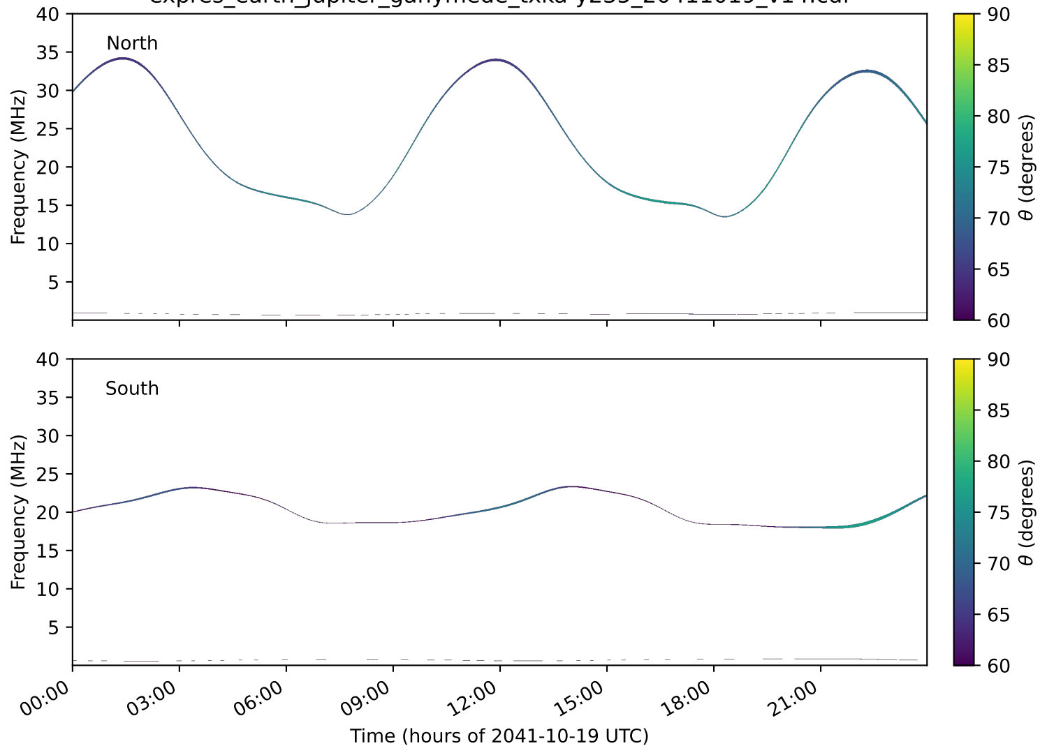
expres_earth_jupiter_ganymede_txka-y235_20411019_v14.cdf
