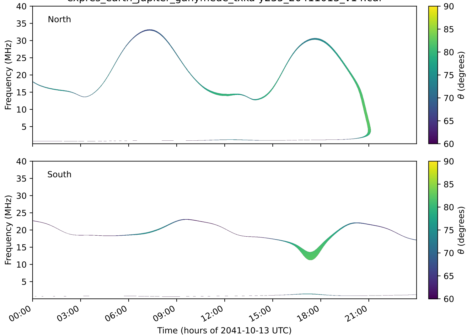
expres_earth_jupiter_ganymede_txka-y235_20411013_v14.cdf
