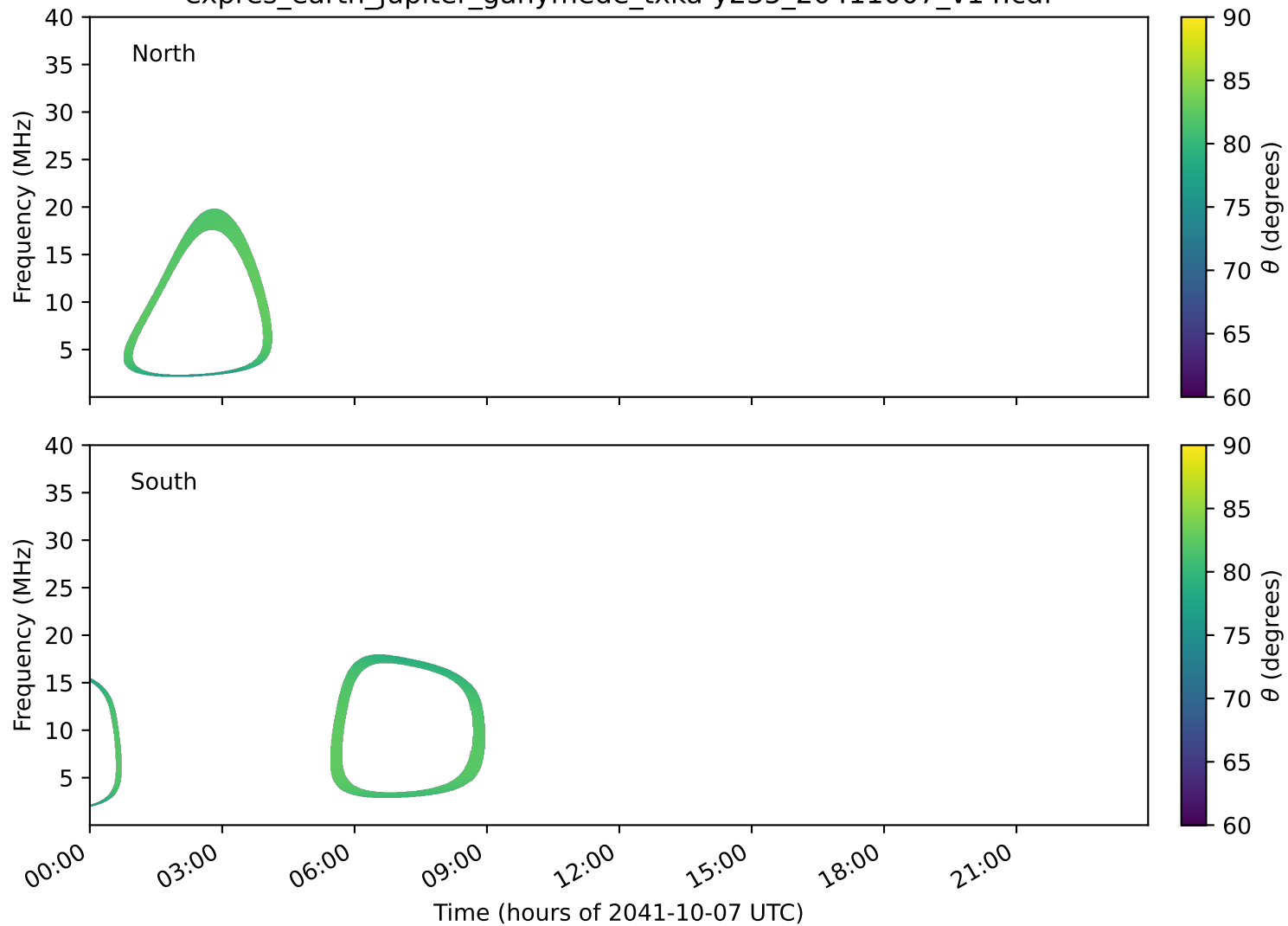
expres_earth_jupiter_ganymede_txka-y235_20411007_v14.cdf
