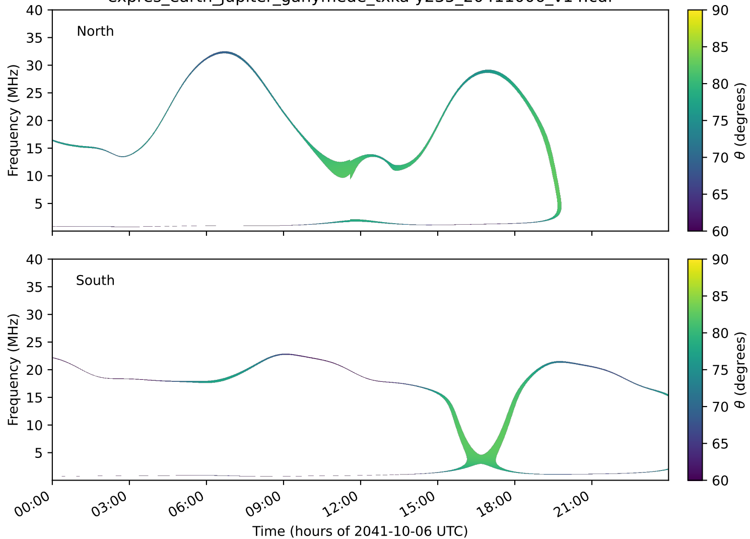
expres_earth_jupiter_ganymede_txka-y235_20411006_v14.cdf
