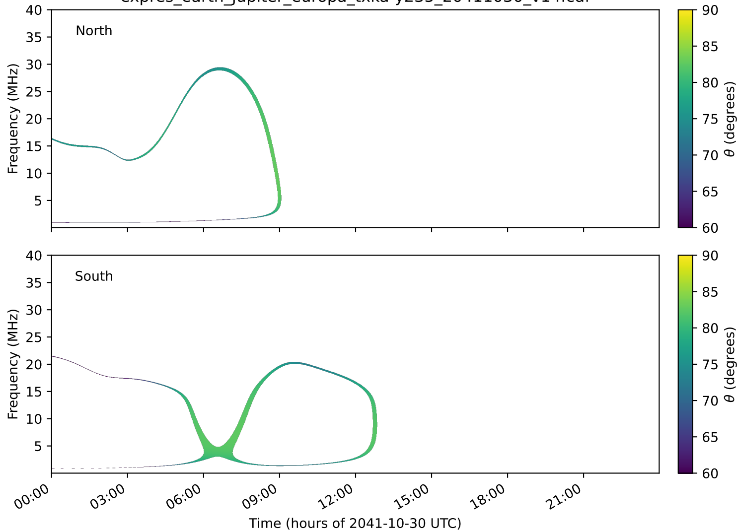
expres_earth_jupiter_europa_txka-y235_20411030_v14.cdf
