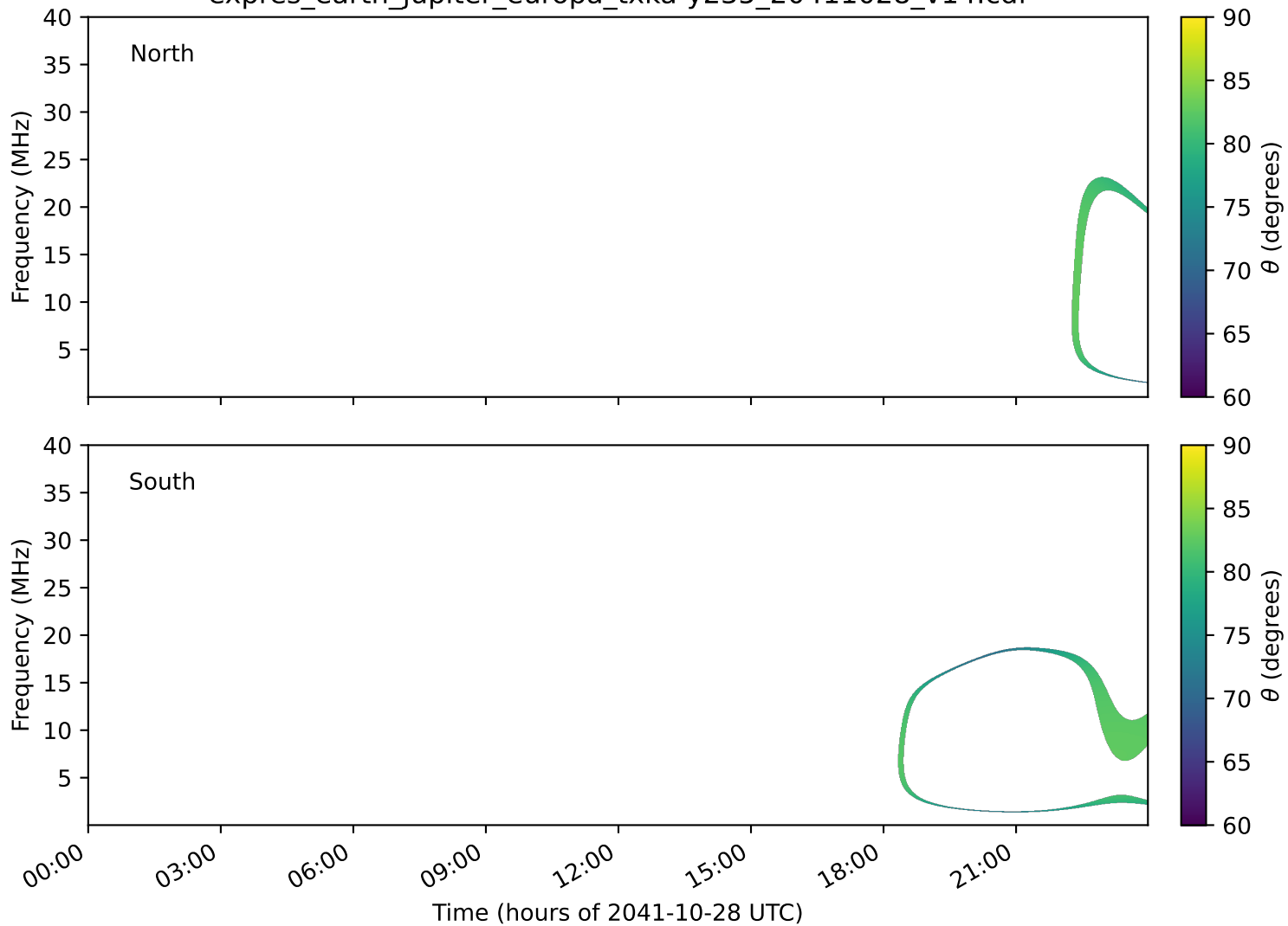
expres_earth_jupiter_europa_txka-y235_20411028_v14.cdf
