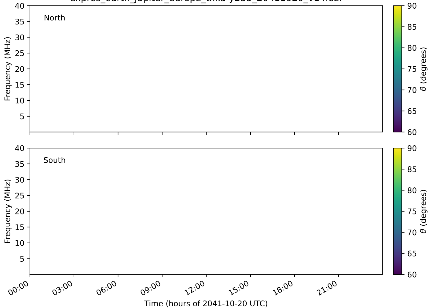
expres_earth_jupiter_europa_txka-y235_20411020_v14.cdf
