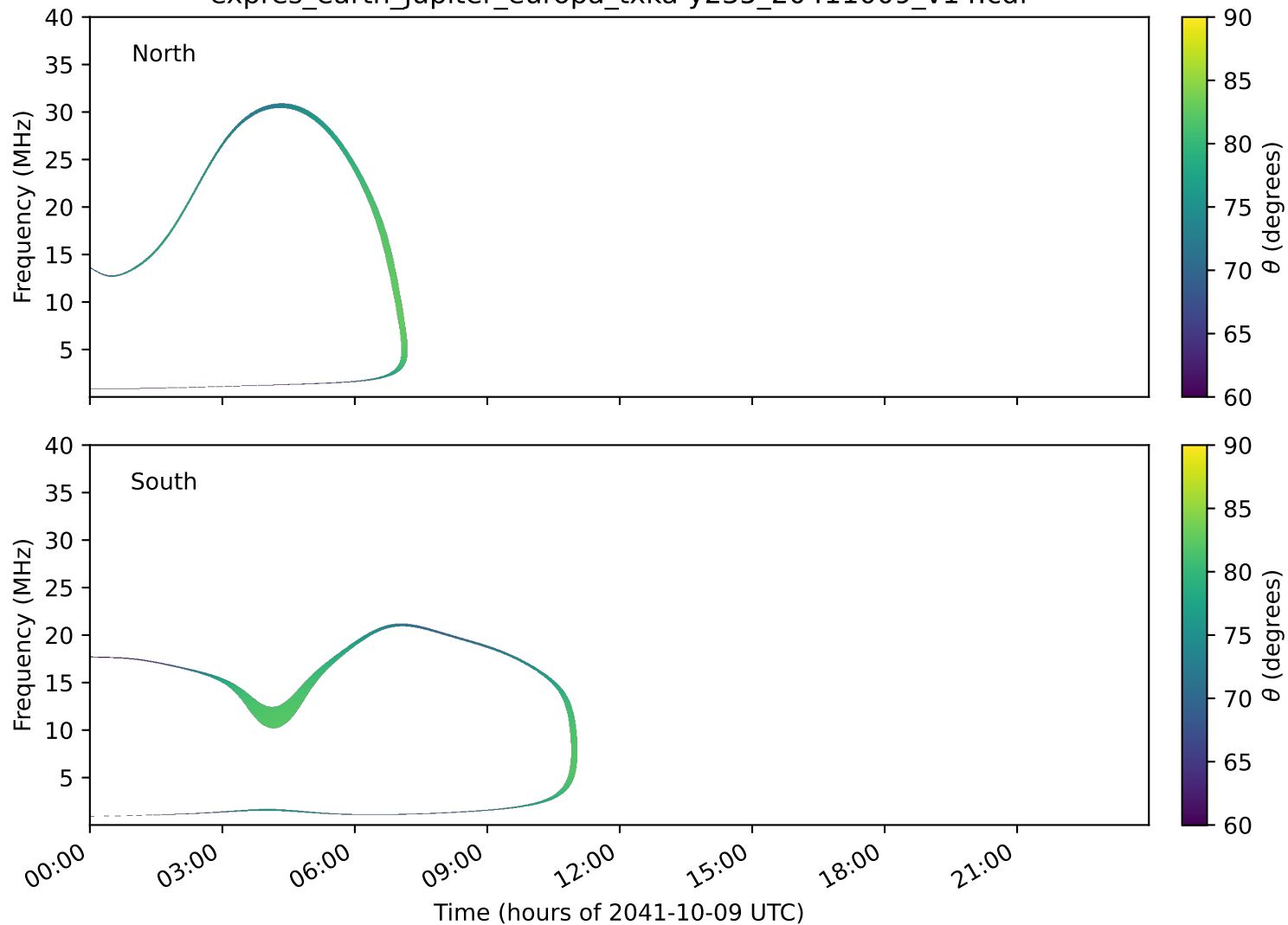
expres_earth_jupiter_europa_txka-y235_20411009_v14.cdf
