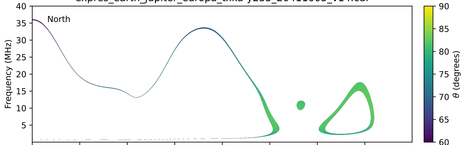
expres_earth_jupiter_europa_txka-y235_20411005_v14.cdf
