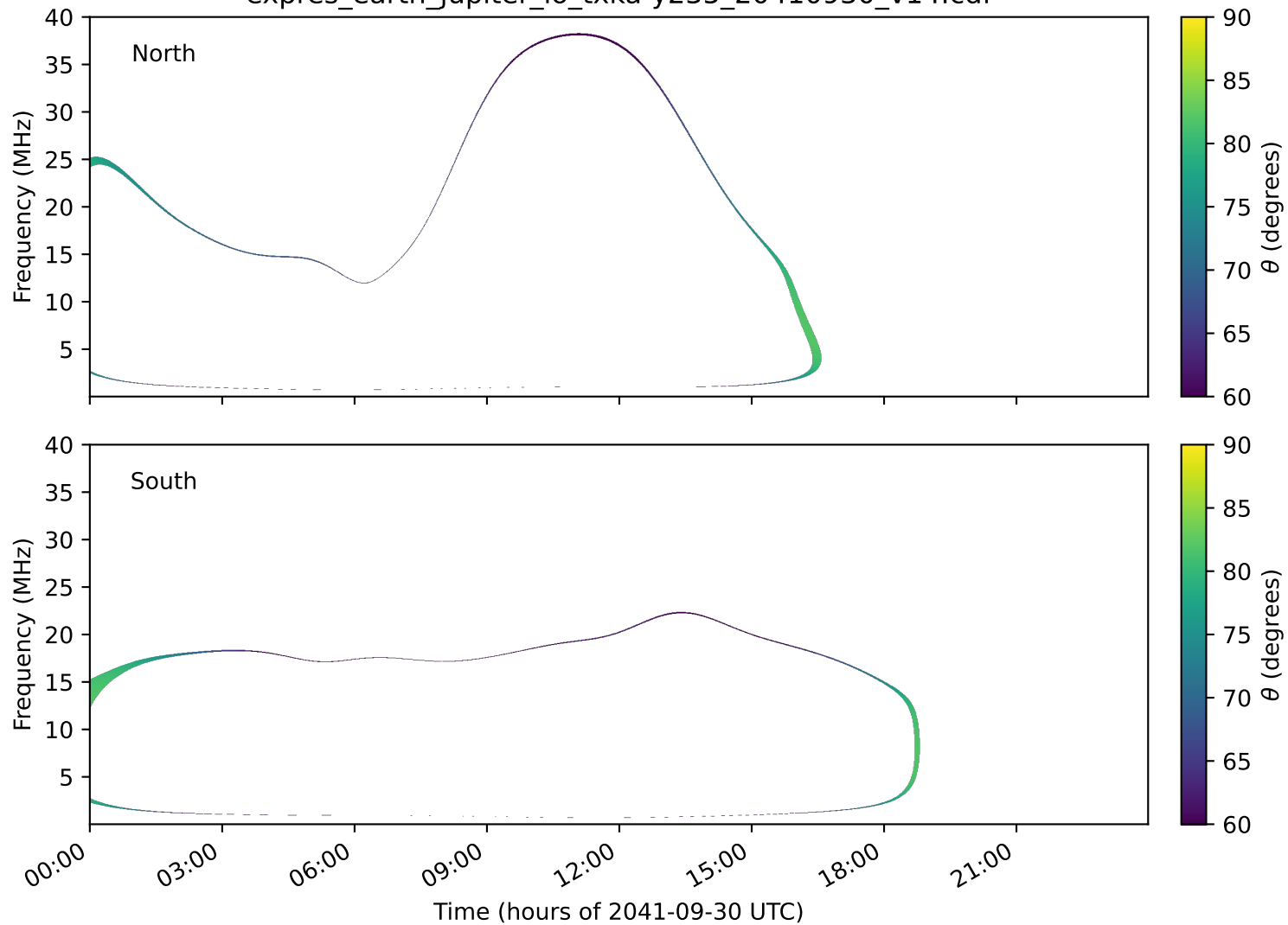
expres_earth_jupiter_io_txka-y235_20410930_v14.cdf
