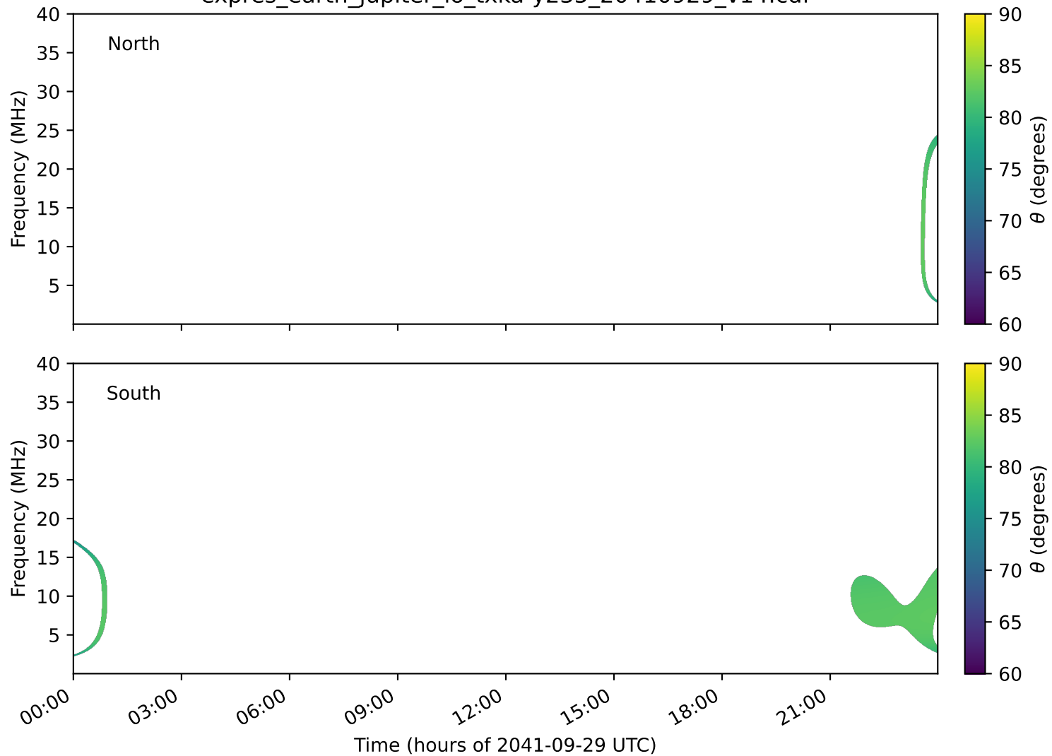
expres_earth_jupiter_io_txka-y235_20410929_v14.cdf
