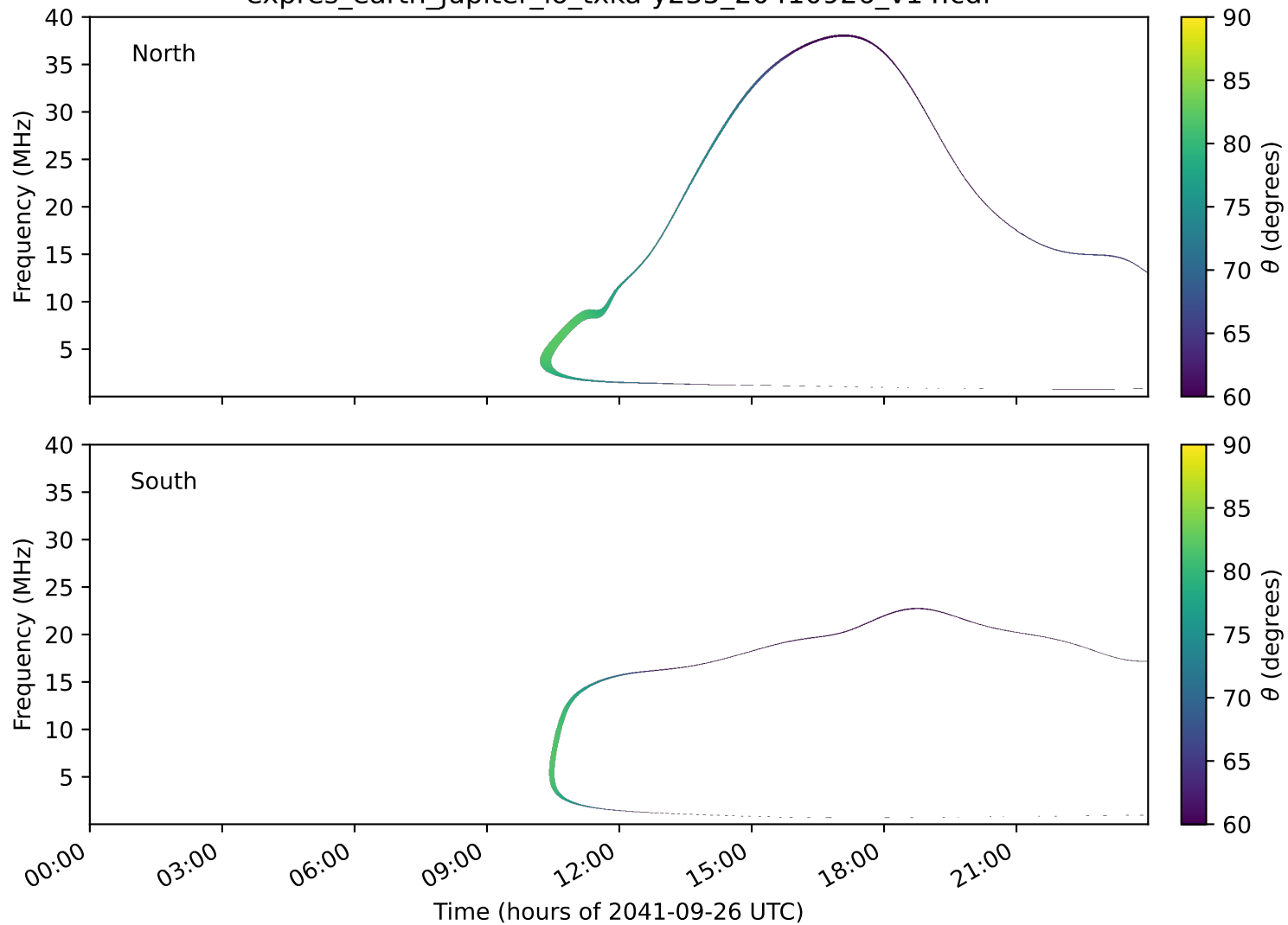
expres_earth_jupiter_io_txka-y235_20410926_v14.cdf
