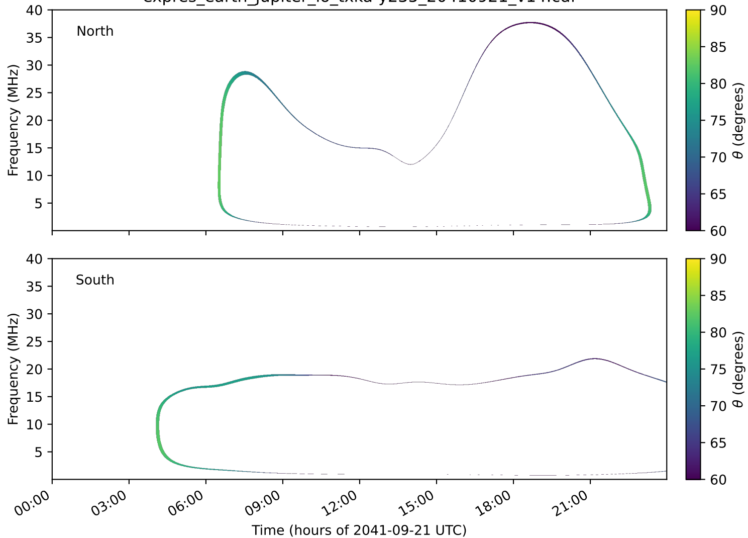
expres_earth_jupiter_io_txka-y235_20410921_v14.cdf
