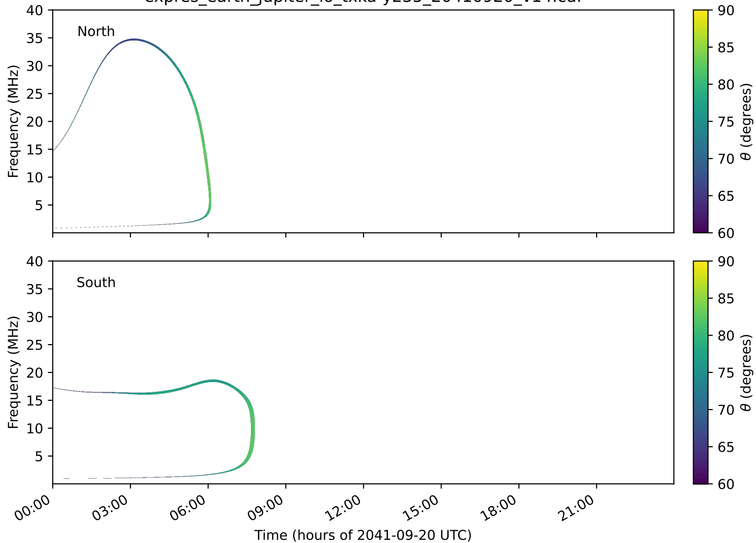
expres_earth_jupiter_io_txka-y235_20410920_v14.cdf
