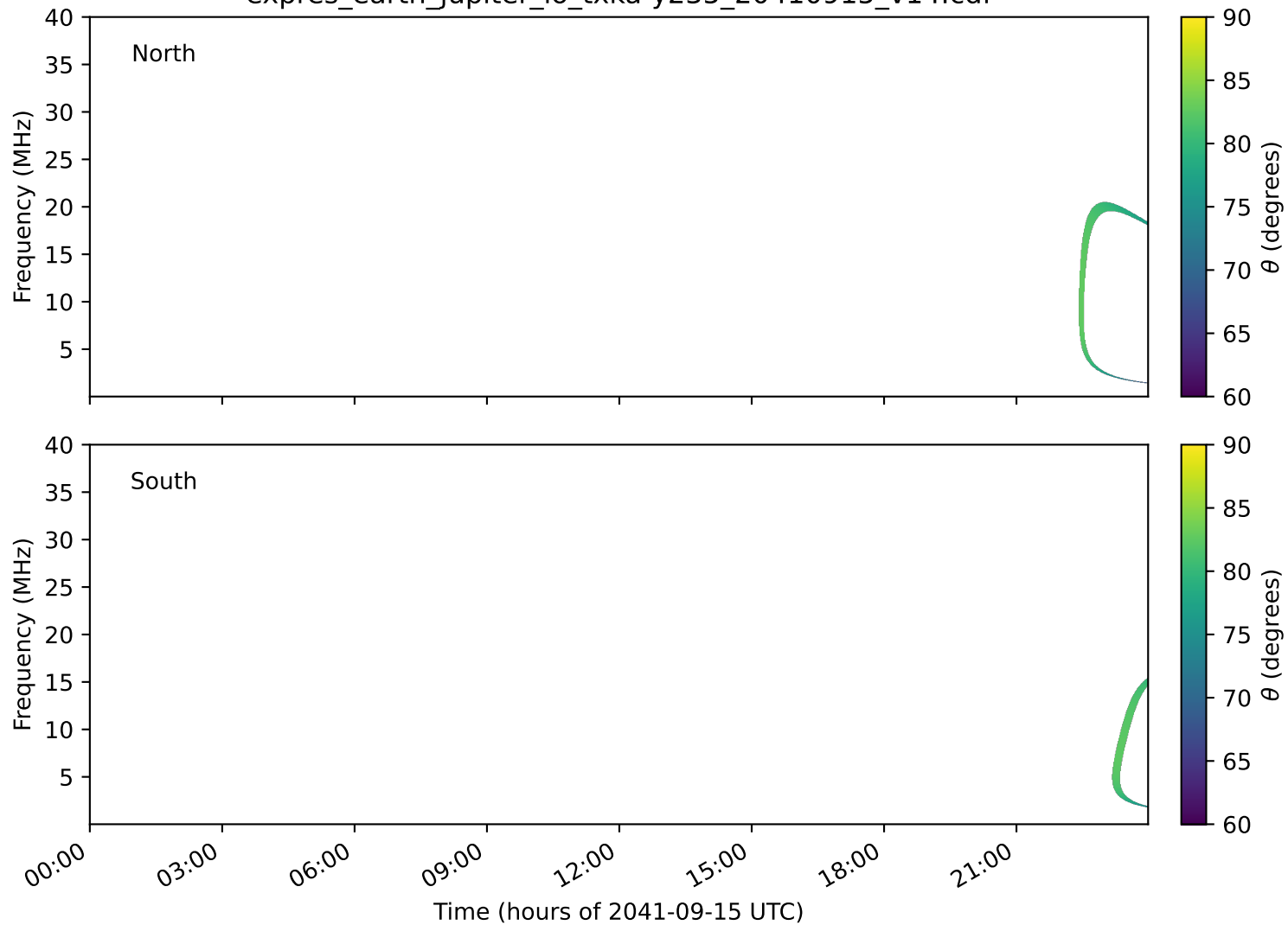
expres_earth_jupiter_io_txka-y235_20410915_v14.cdf
