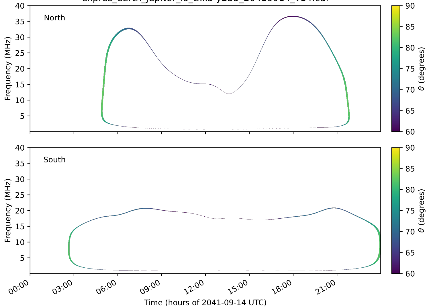
expres_earth_jupiter_io_txka-y235_20410914_v14.cdf
