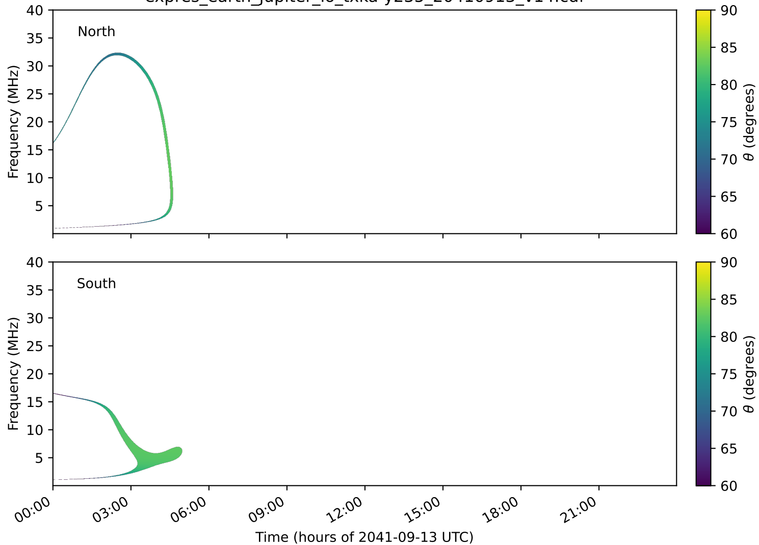
expres_earth_jupiter_io_txka-y235_20410913_v14.cdf
