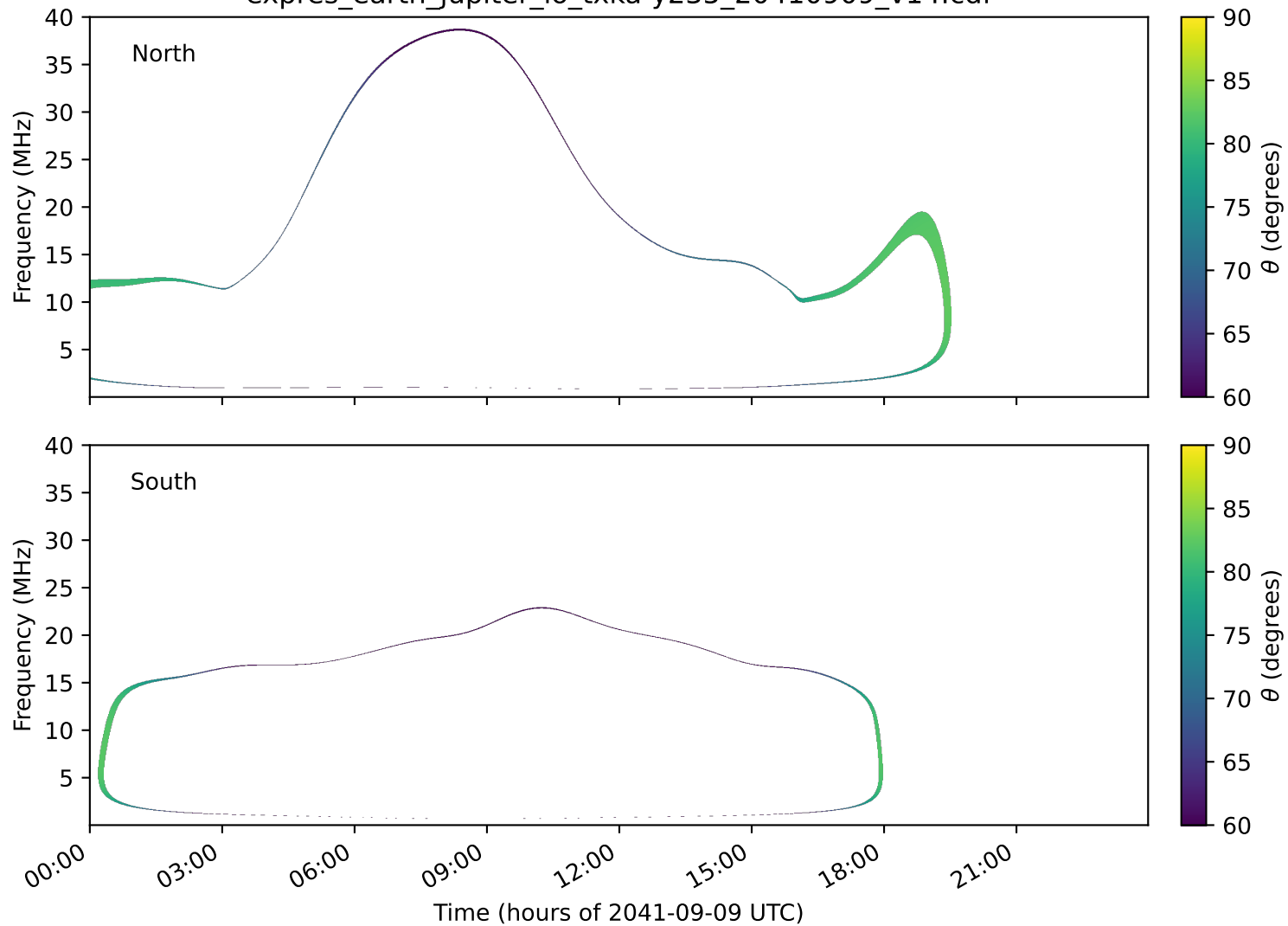
expres_earth_jupiter_io_txka-y235_20410909_v14.cdf
