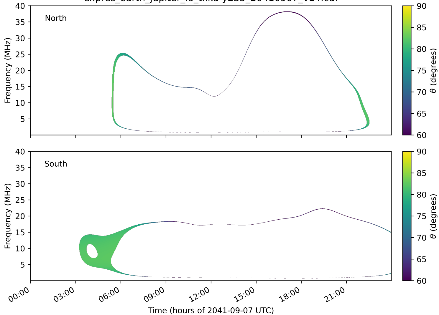
expres_earth_jupiter_io_txka-y235_20410907_v14.cdf
