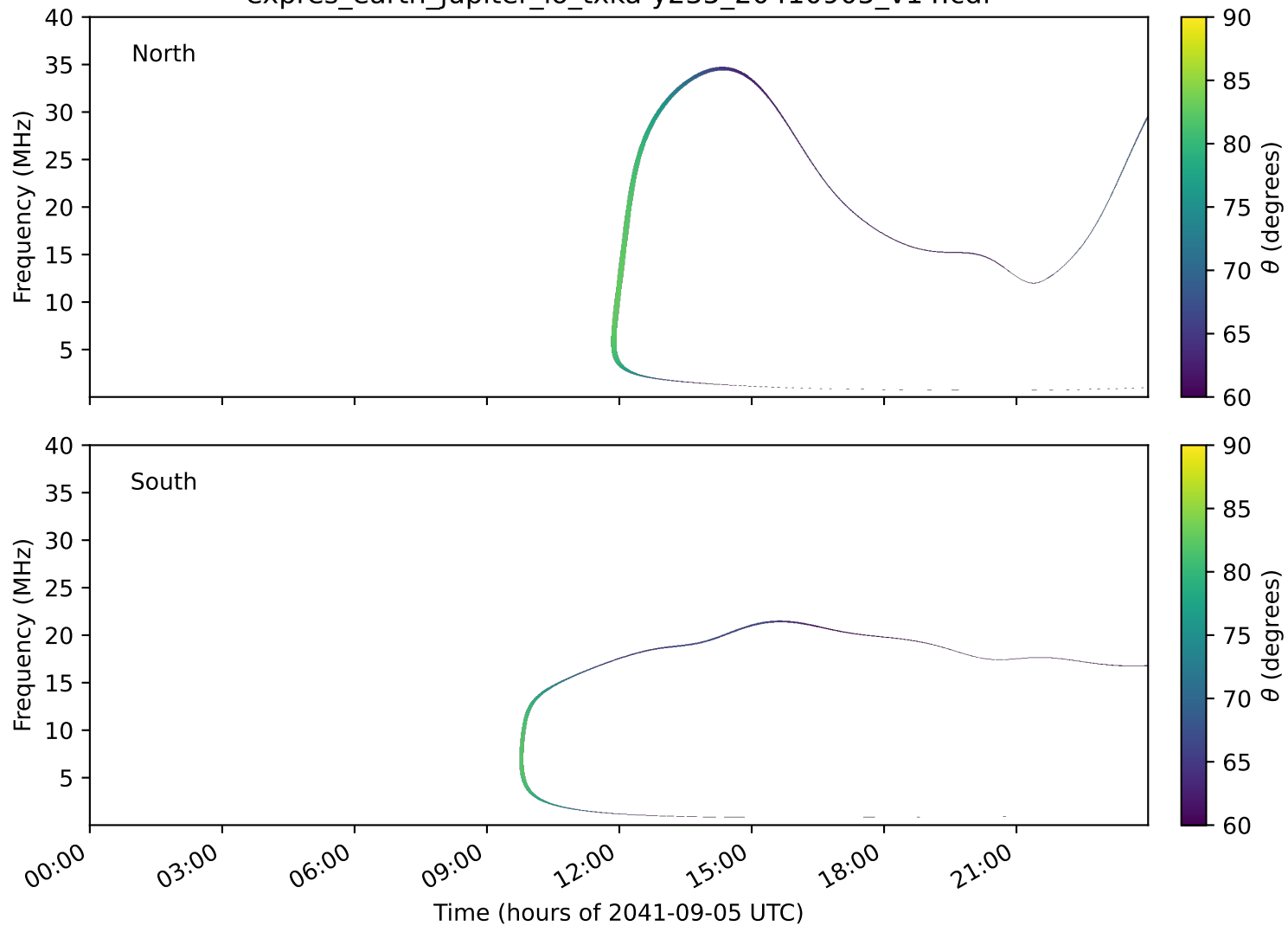
expres_earth_jupiter_io_txka-y235_20410905_v14.cdf
