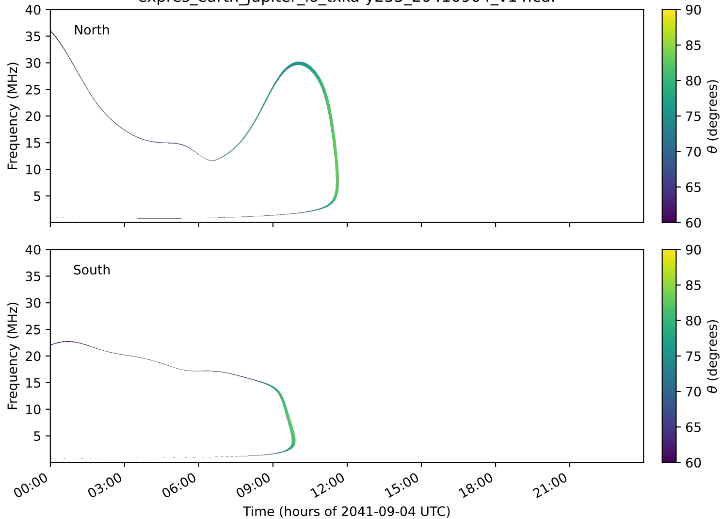
expres_earth_jupiter_io_txka-y235_20410904_v14.cdf
