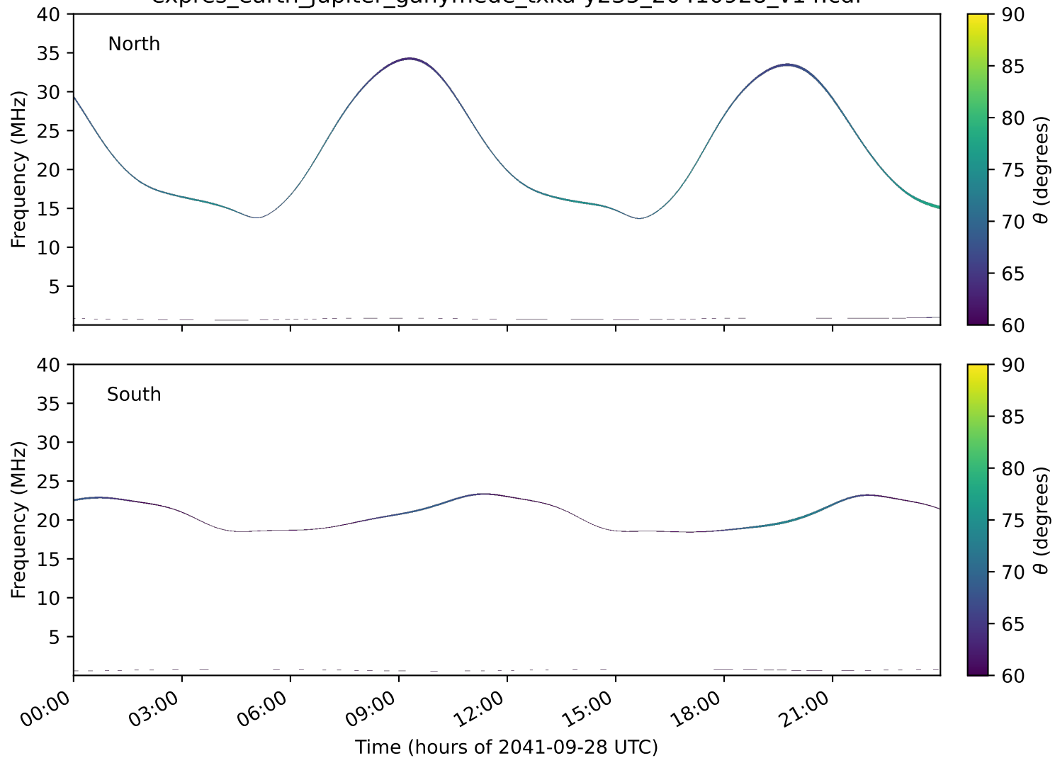
expres_earth_jupiter_ganymede_txka-y235_20410928_v14.cdf
