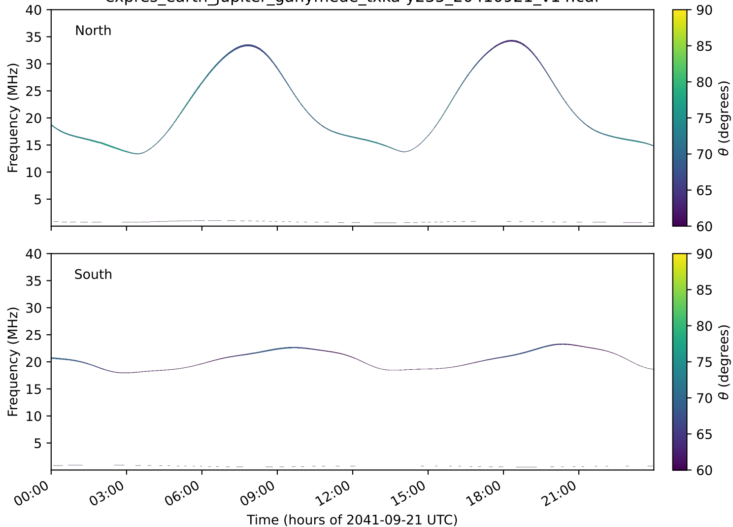
expres_earth_jupiter_ganymede_txka-y235_20410921_v14.cdf
