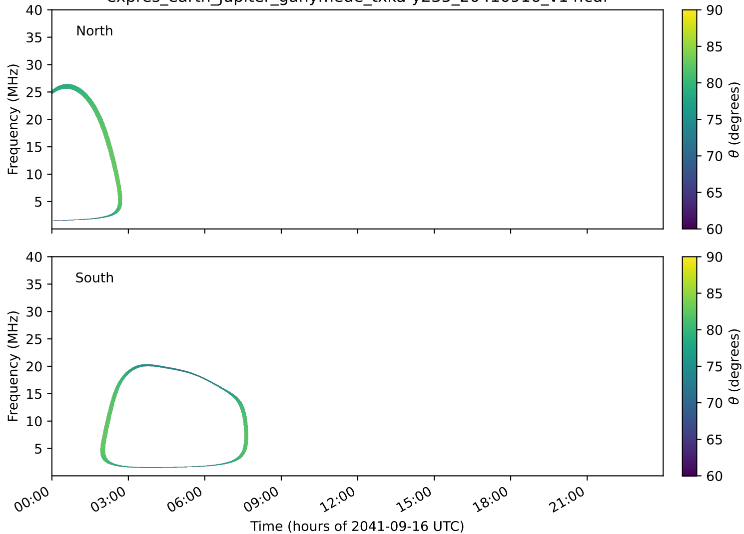
expres_earth_jupiter_ganymede_txka-y235_20410916_v14.cdf
