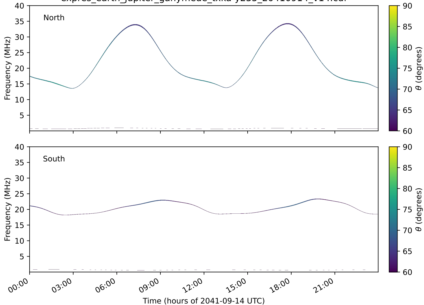
expres_earth_jupiter_ganymede_txka-y235_20410914_v14.cdf
