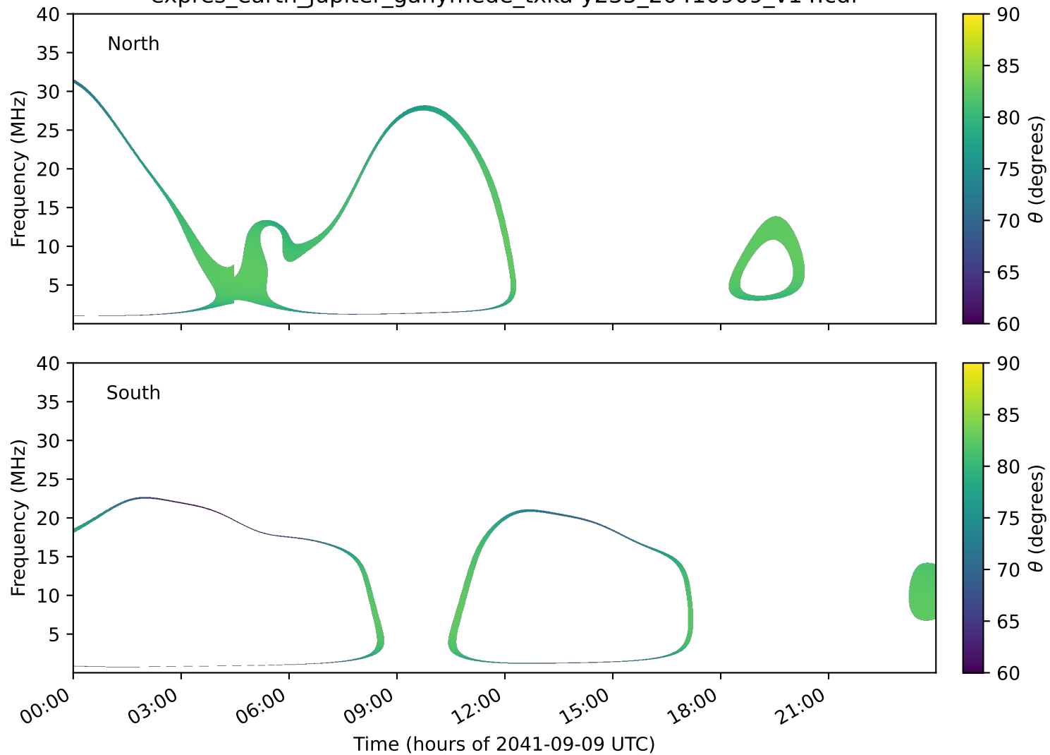
expres_earth_jupiter_ganymede_txka-y235_20410909_v14.cdf
