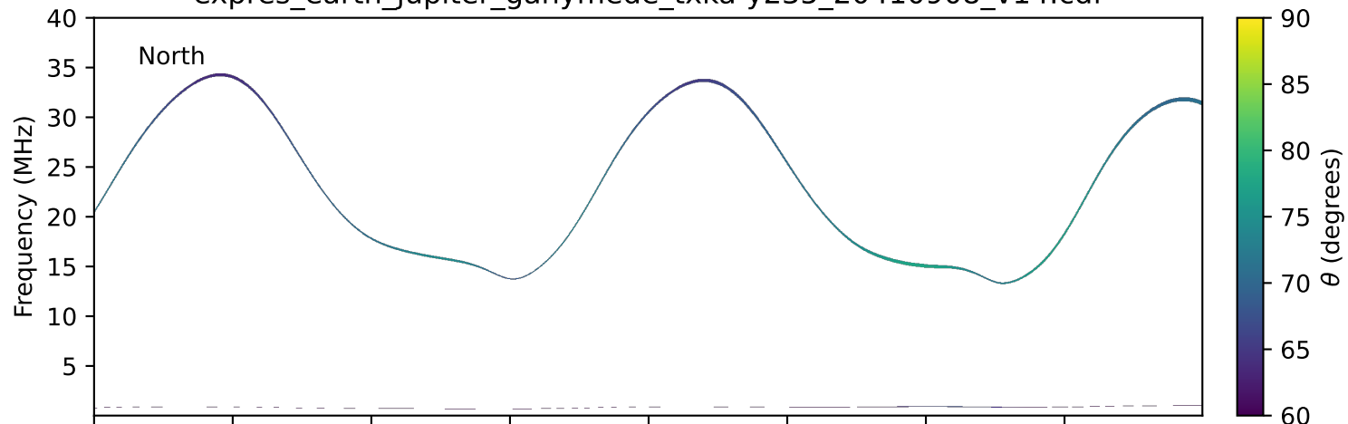
expres_earth_jupiter_ganymede_txka-y235_20410908_v14.cdf
