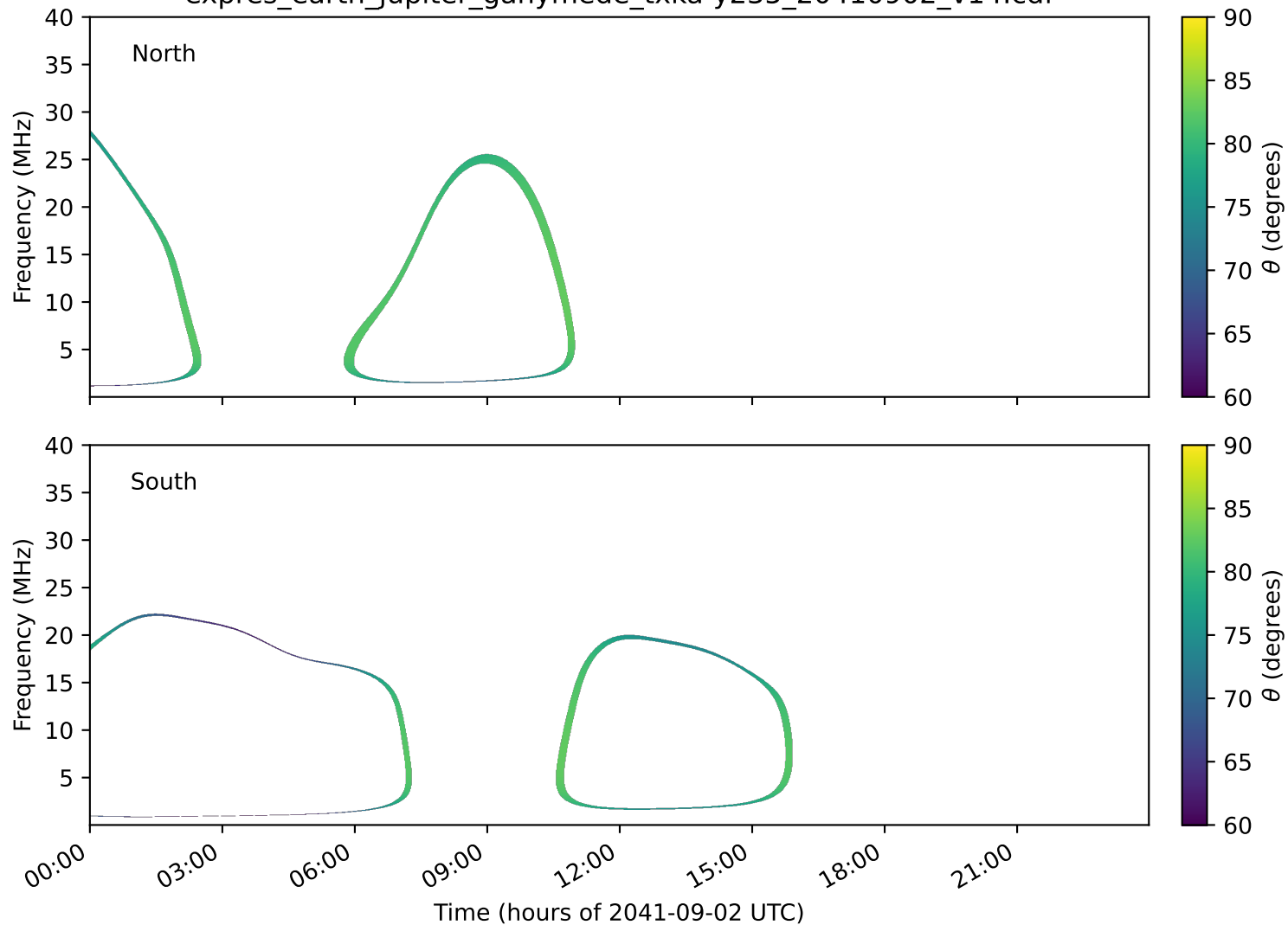
expres_earth_jupiter_ganymede_txka-y235_20410902_v14.cdf
