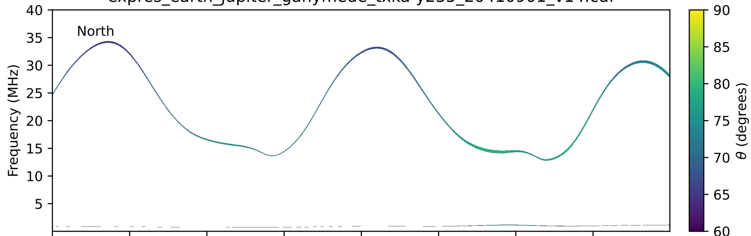
expres_earth_jupiter_ganymede_txka-y235_20410901_v14.cdf
