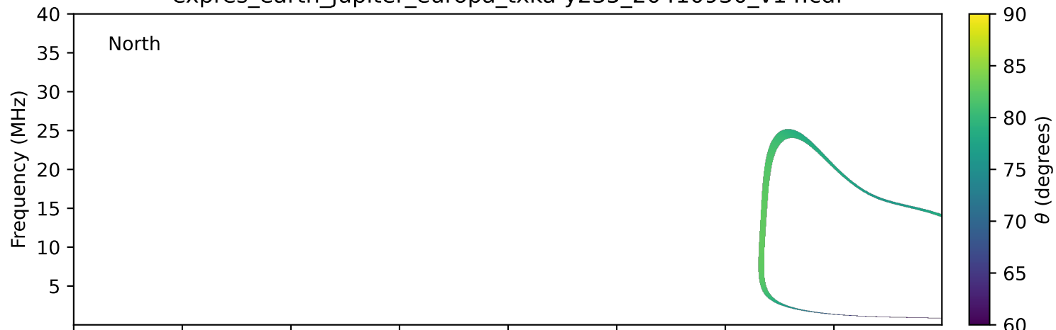
expres_earth_jupiter_europa_txka-y235_20410930_v14.cdf
