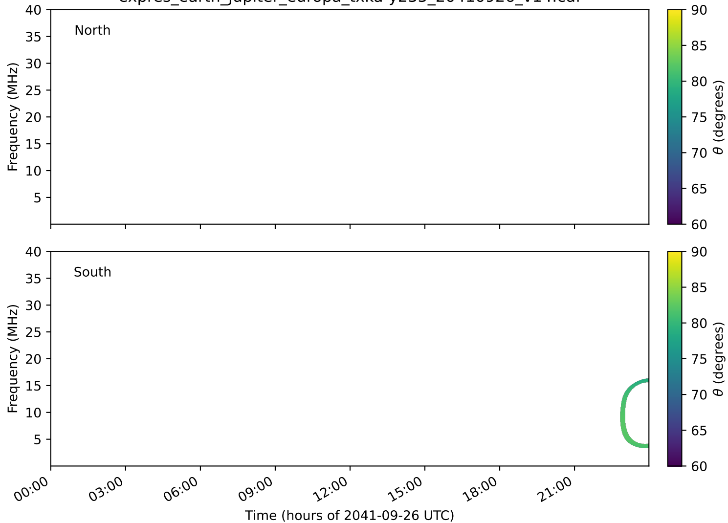
expres_earth_jupiter_europa_txka-y235_20410926_v14.cdf
